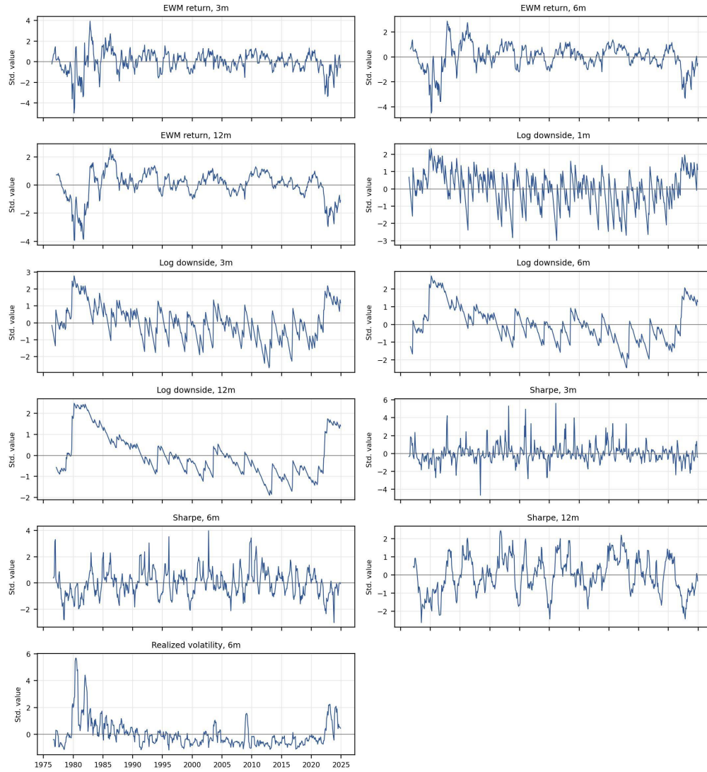
Figure C.18: Bond teacher features.
