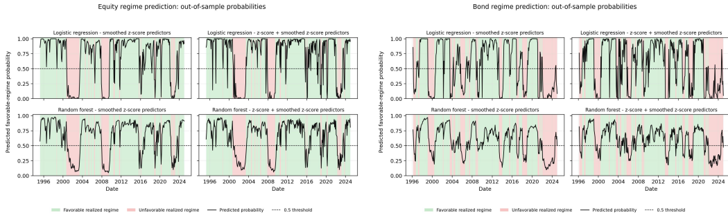
Figure 3: INDEPENDENT student out-of-sample probability paths. The left panel reports equity favourable-regime probabilities, and the right panel reports bond favourable-regime probabilities. Shading marks the realised teacher label, the black line reports the predicted favourable-regime probability, and the dashed line marks the 0.5 threshold.
