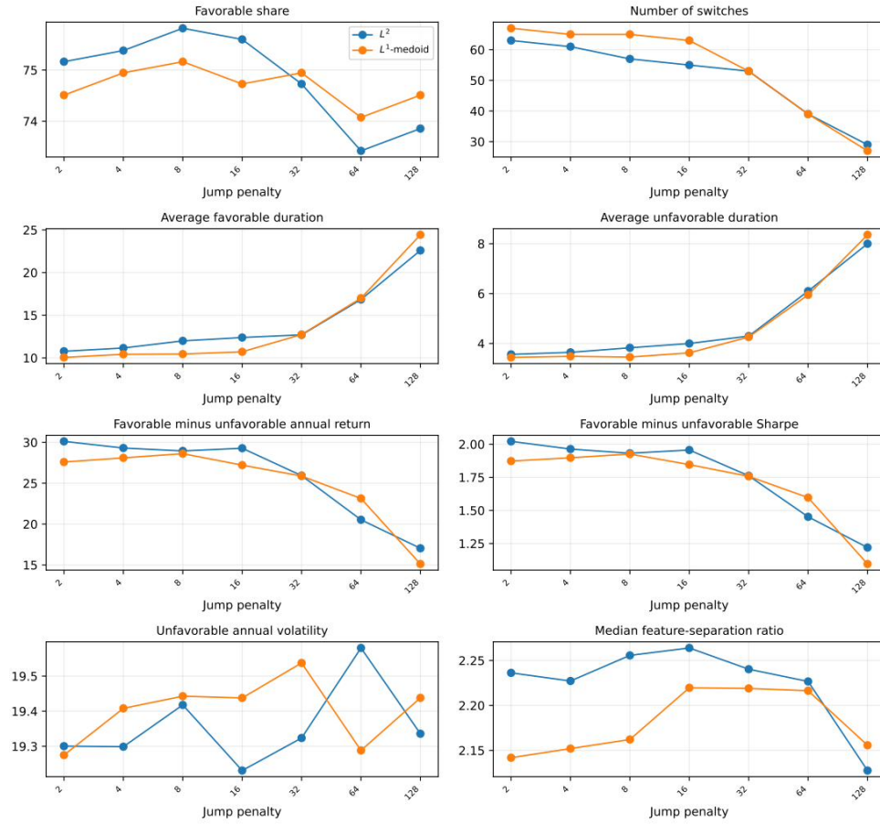
Figure C.13: Equity regime label: jump-penalty diagnostics.
