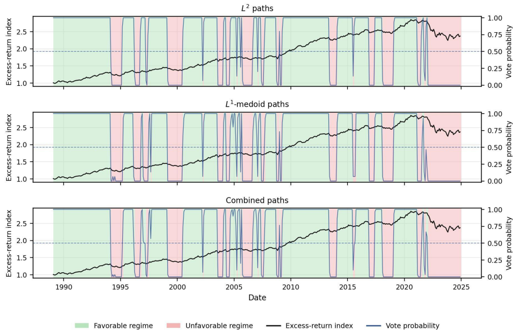
Figure C.16: Bond regime label: majority-vote construction.
