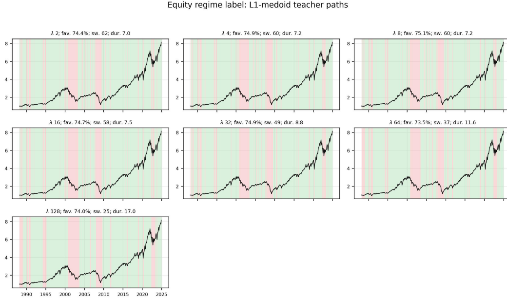
Figure C.10: Equity regime label: L^1 -medoid teacher paths.
