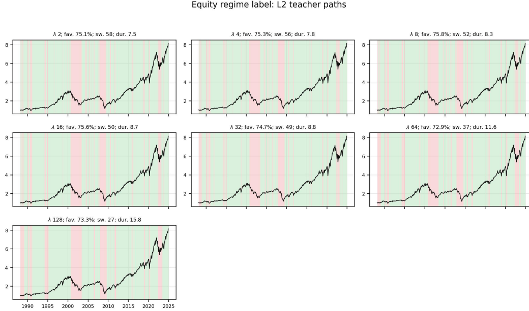
Figure C.9: Equity regime label: L^2 teacher paths.
