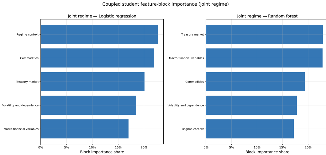
Figure 6: COUPLED student feature-block importance for the three-class next-month regime forecast. Logistic-regression importance is based on absolute coefficient magnitude; random-forest importance is impurity-based; values are aggregated within predictor blocks.
