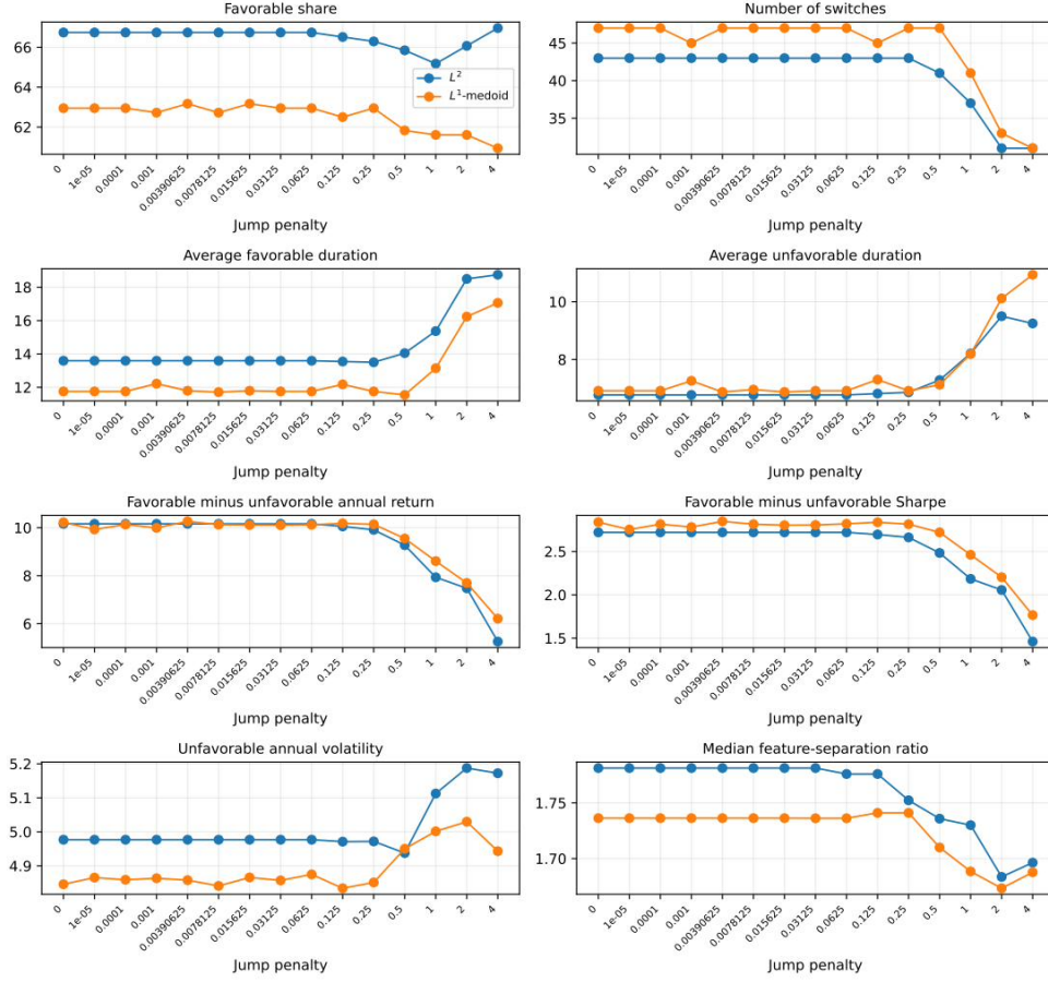
Figure C.14: Bond regime label: jump-penalty diagnostics.
