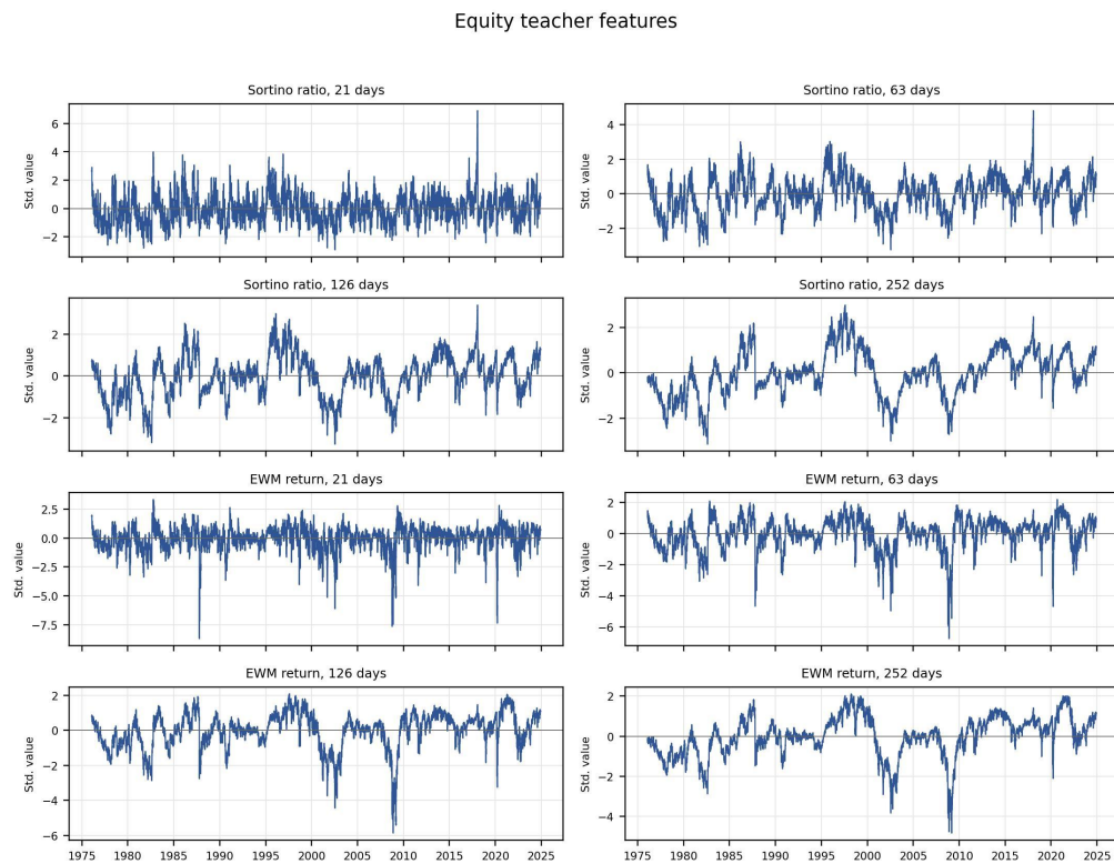
Figure C.17: Equity teacher features.
