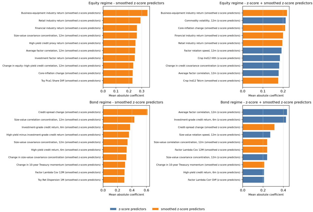
Figure F.30: Student prediction individual predictor importance.
